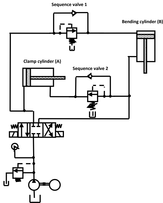
Figure 1.7 Sequencing circuit.
