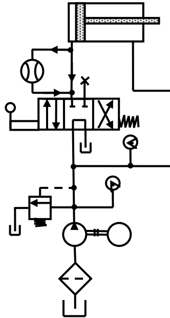
Figure 1.3 Regenerative circuit.
