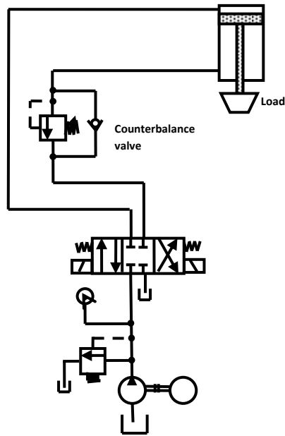
Figure 1.6 Counterbalance valve circuit.
