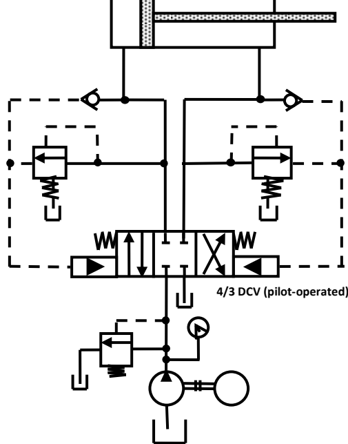
Figure 1.8 Sequencing circuit.
