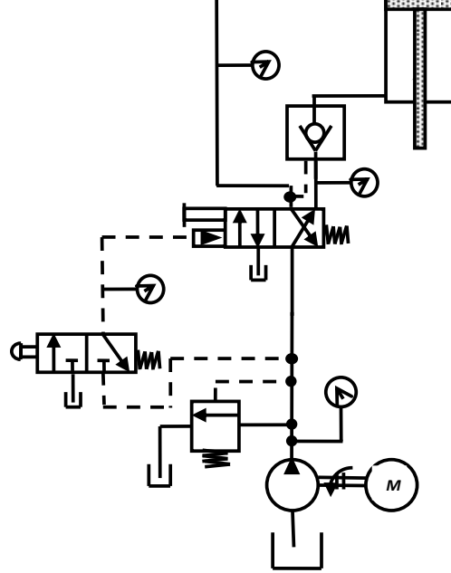
Figure 1.13 Fail-safe circuits – inadvertent cylinder extension.
