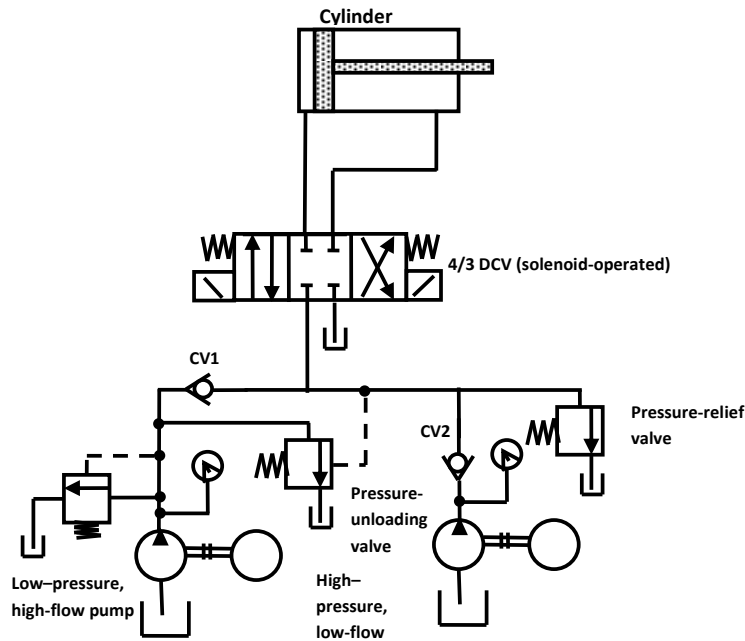
Figure 1.5 Double-pump circuit.
