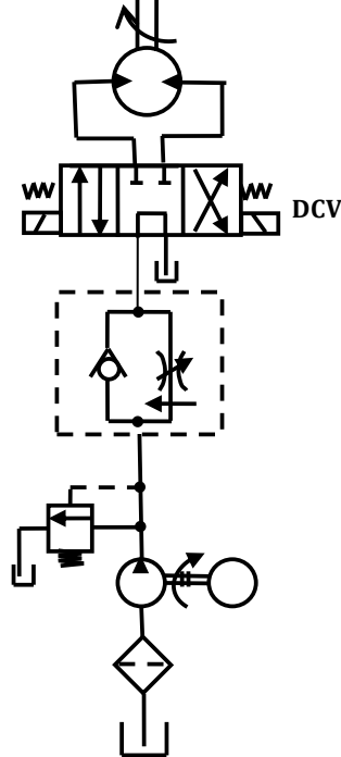
Figure 1.12 Speed control of a motor.
